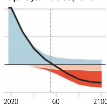
Higher residual emissions require yet more CO 2 removal
