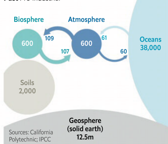
Total carbon stocks and annual flows, gigatonnes of carbon
