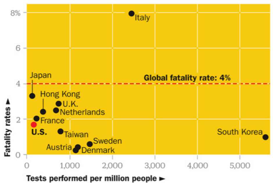
COVID-19 case fatality vs. testing rates
