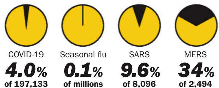
Fatalities as a percentage of all cases
