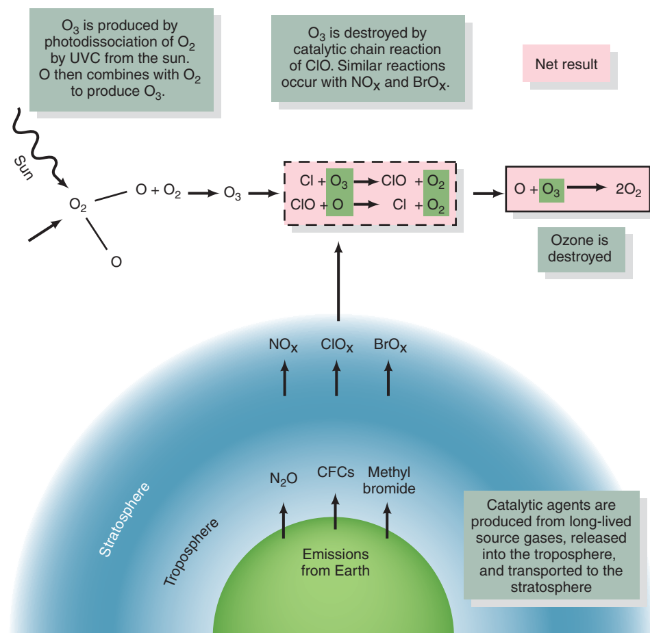
FIGURE 21.15 Processes of natural formation of ozone and destruction by CFCs, N 2 O, and methyl bromide. (Source: Modified from NASA-GSFC, "Stratospheric Ozone," accessed August 22, 2000, at http://see.gsfc.nasa.gov .)
