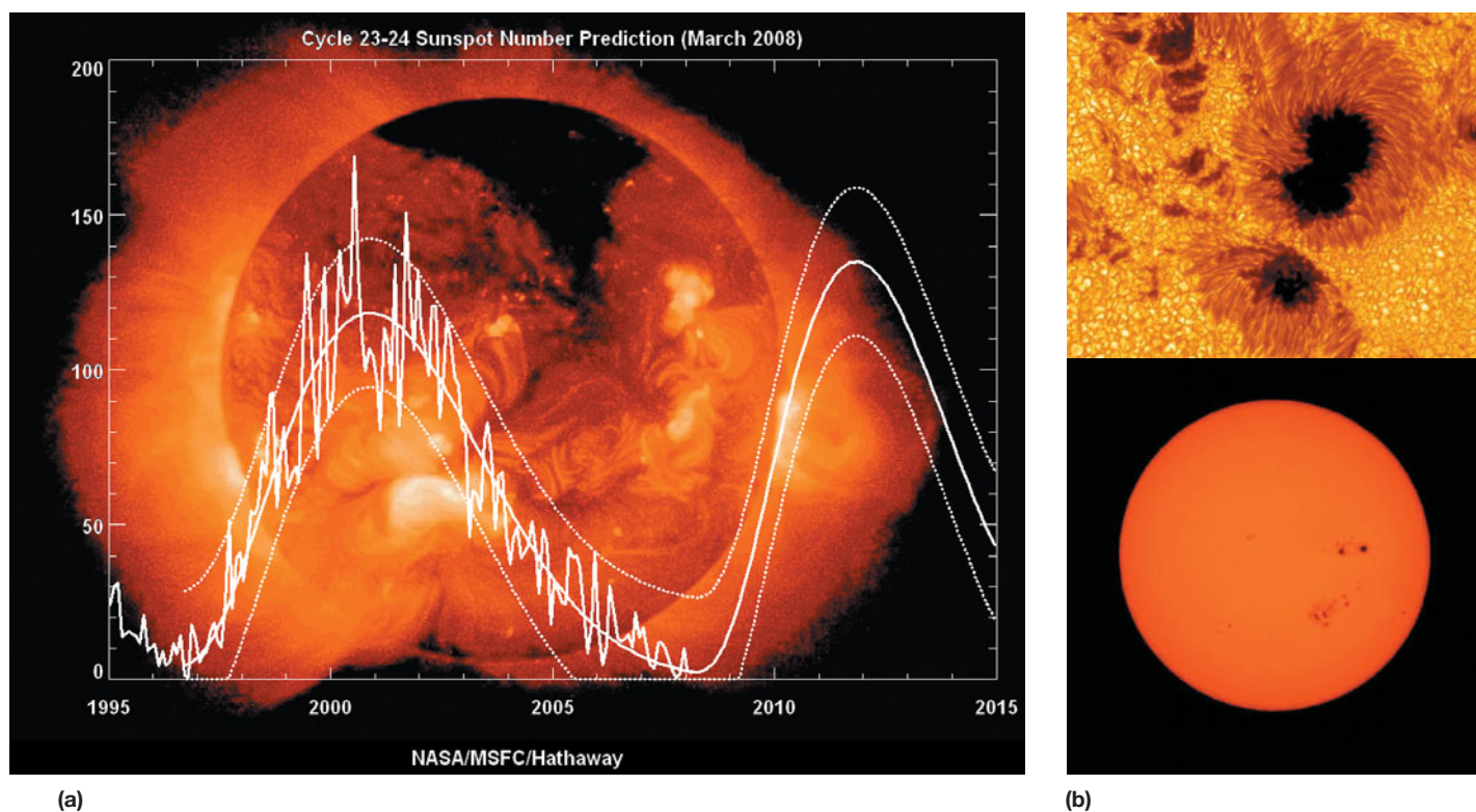
FIGURE 20.14 (a) Sunspot cycle with number of sunspots per year, from 1995 to 2009 and (b) photos of sunspots in 2003. The large sunspots are about 150,000 km across (for comparison, Earth's diameter is about 12,750 km). The sunspots are the dark areas, and each is surrounded by an orange ring and then a hot gold color. Notice the great variety in the number of sunspots from year to year in the 11-year cycle (over 150 in 2001 and very few in 2008 and 2009). (Source: NOAA Images.)
