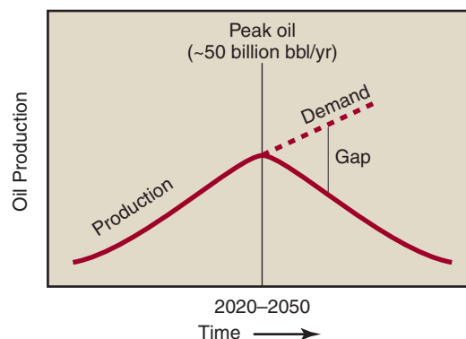
FIGURE 15.2 Idealized diagram of world oil production and peak between 2020 and 2050. When production cannot meet demand, a gap (shortage) develops.
