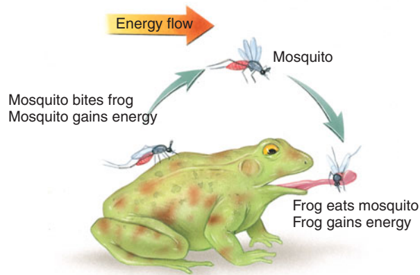
FIGURE 5.12 An impossible ecosystem. Energy always changes from a more useful, more highly organized form to a less useful, disorganized form. That is, energy cannot be completely recycled to its original state of organized, high-quality usefulness. For this reason, the mosquito–frog system will eventually stop when not enough useful energy is left. (There is also a more mundane reason: Only female mosquitoes require blood, and then only in order to reproduce. Mosquitoes are otherwise herbivorous.)
