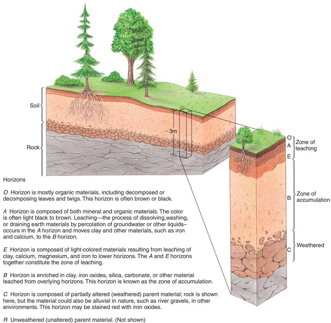
FIGURE 11.14 Idealized diagram of a soil, showing soil horizons.
