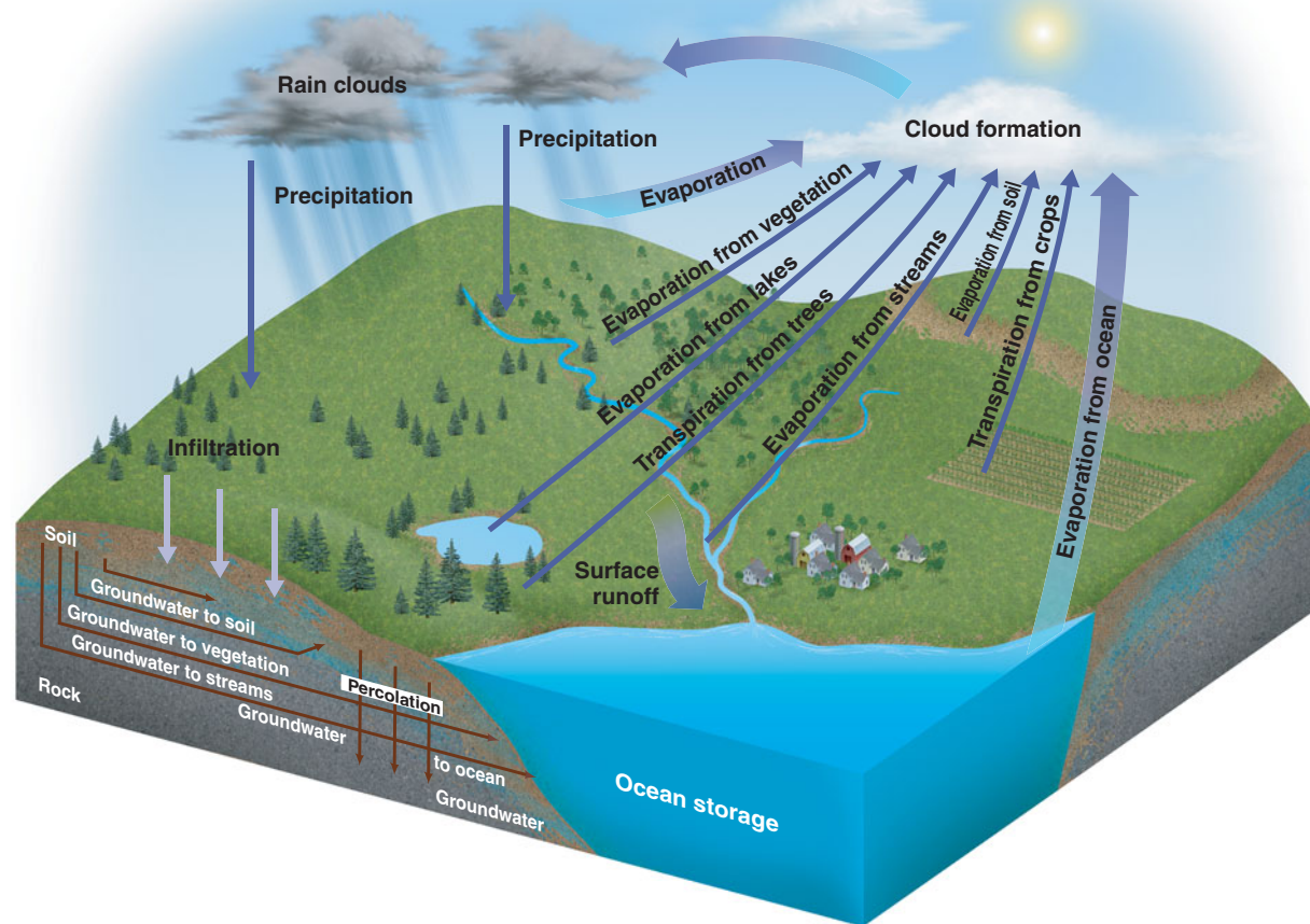
FIGURE 18.2 The hydrologic cycle, showing important processes and transfer of water. (Source: Modified from Council on Environment Quality and Department of State, The Global 2000 Report to the President , vol. 2 [Washington, DC].)
