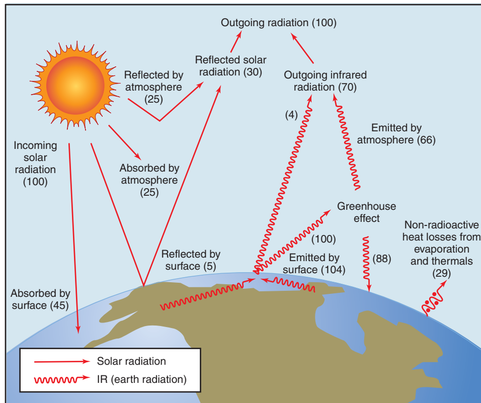
FIGURE 20.17 Idealized diagram showing Earth's energy balance and the greenhouse effect. Incoming solar radiation is arbitrarily set at 100 units, and this is balanced by outgoing radiation of 100 units. Notice that some of the fluxes (rates of transfer) of infrared radiation (IR) are greater than 100, reflecting the role of the greenhouse effect. Some of these fluxes are explained in the diagram. (Source: Modified from D.I. Hartmann, Global Physical Climatology , International Geophysics Series, vol. 56 [New York: Academic Press, 1994] and S. Schneider, "Climate Modeling," Scientific American 256 No. 5.)
