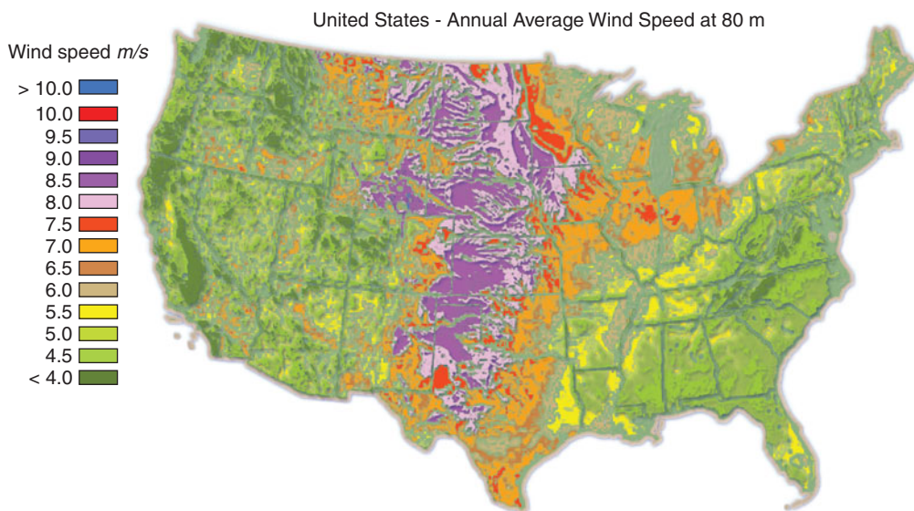
FIGURE 16.13 Wind energy potential in the United States.
