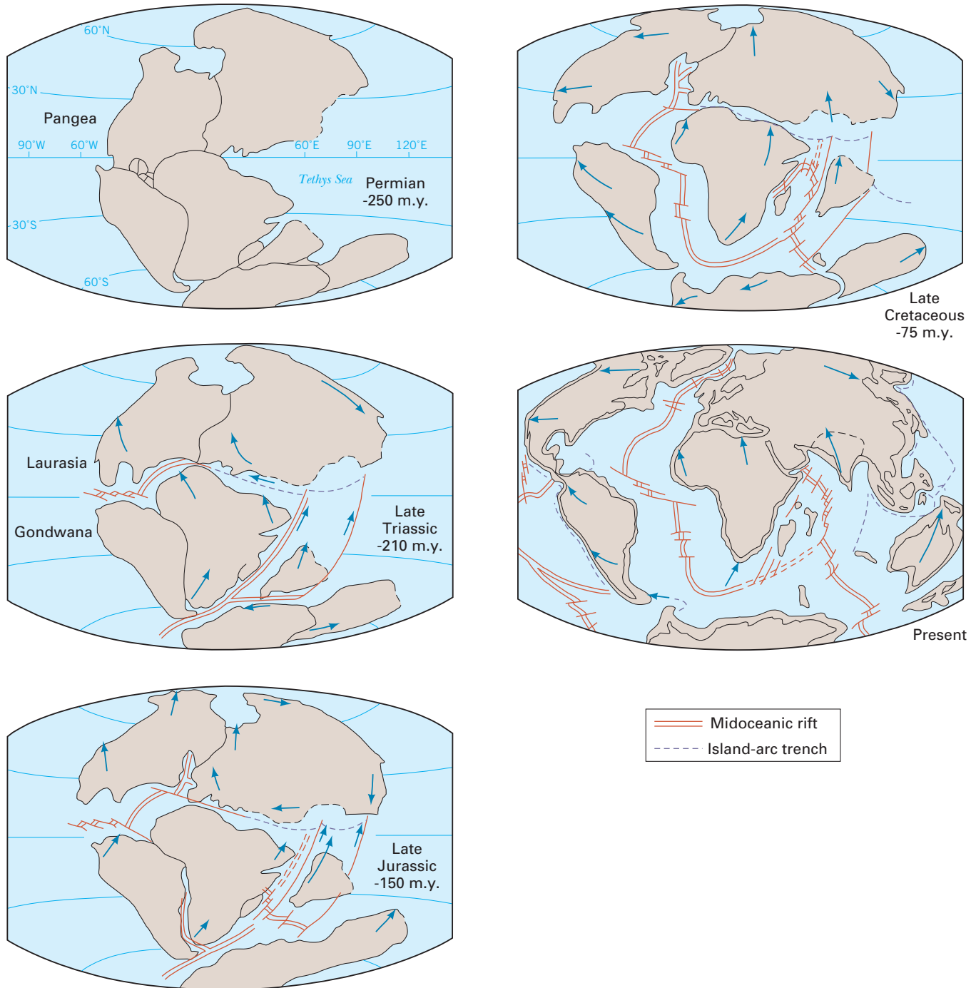
Figure 13.3 Wegener's Hypothesis of Continental Drift. Wegener's dates have been revised but were remarkably prescient. Adapted with permission from: Wegener, The Origin of the Continents and Oceans , 1914.
