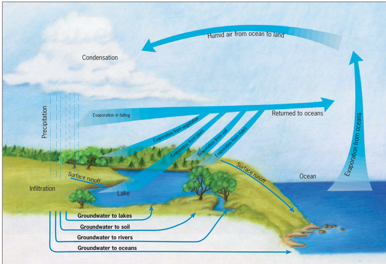
Figure 13.10 The Hydrologic Cycle. The hydrologic cycle shows water carried from the oceans and from other water bodies over land, where precipitation, runoff, and evapotranspiration sustain the system. © E. H. Fouberg, A. B. Murphy, H. J. de Blij, and John Wiley & Sons, Inc.
