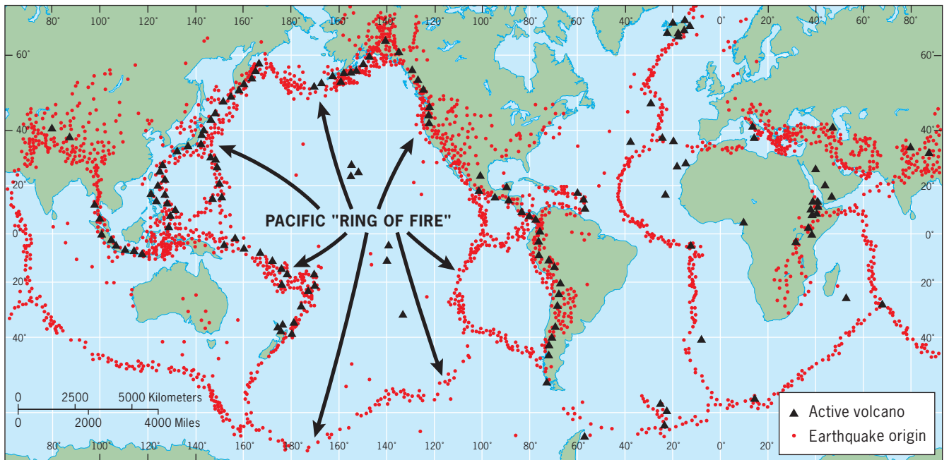
Figure 13.5 Recent Earthquakes and Volcanic Eruptions. © H. J. de Blij, P. O. Muller, and John Wiley & Sons, Inc.
