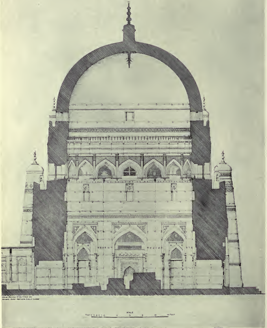
TOMB OF SHAH RUKN-I-ALAM MULTAN CROSS SECTION
