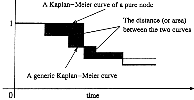
Fig. 142 Wasserstein metrics.
