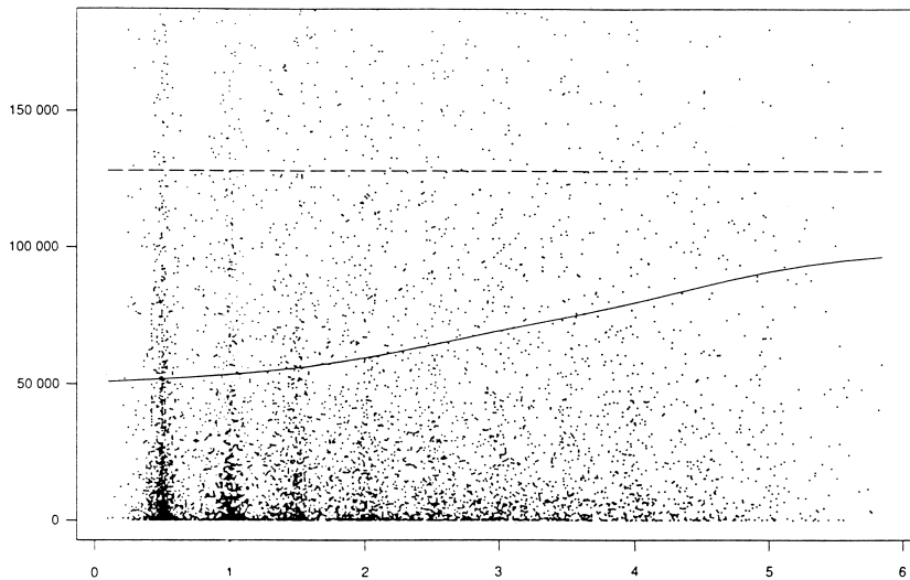
Fig. 138 Variogram plots.
