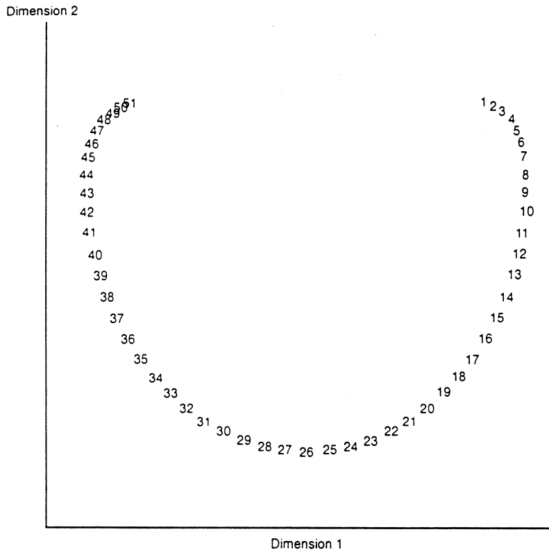
Fig. 119 Horseshoe effect.
