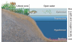
FIGURE 5.20 The layers of a deep lake are determined mainly by gradients of light, oxygen, and temperature. The epilimnion is affected by surface mixing from wind and thermal convections, while mixing between the hypolimnion and epilimnion is inhibited by a sharp temperature and density difference at the thermocline.
