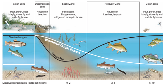
FIGURE 18.6 Oxygen sag downstream of an organic source. A great deal of time and distance may be required for the stream and its inhabitants to recover.
