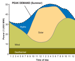
FIGURE 20.31 The wind doesn't blow all the time, nor is sunshine always available, but a mix of renewable resources could supply all the energy we need, especially if distant facilities are linked together. This graph shows hypothetical energy supplies for a typical July day in California.
