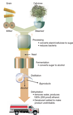
FIGURE 20.22 Ethanol (or ethyl alcohol) can be produced from a wide variety of sources. Maize (corn) and other starch grains are milled (ground) and then processed to convert starch to sugar, which can be fermented by yeast into alcohol. Distillation removes contaminants and yields pure alcohol. Cellulosic crops, such as wood or grasses, can also be converted into sugars, but the process is more difficult. Steam blasting, alkaline hydrolysis, enzymatic conditioning, and acid pretreatment are a few of the methods for breaking up woody material. Once sugars are released, the processes are similar.
