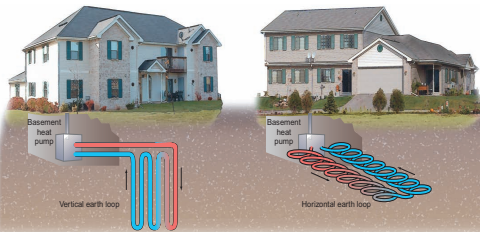
FIGURE 20.32 Geothermal energy can cut heating and cooling costs by half in many areas. In summer (shown here), warm water is pumped through buried tubing (earth loops) where it is cooled by constant underground temperatures. In winter, the system reverses and the relatively warm soil helps heat the house. Where space is limited (left), earth loops can be vertical. If more space is available (right) the tubing can be laid in shallow horizontal trenches. A heat exchanger concentrates heat, so water entering the house is far warmer than the ground temperature.
