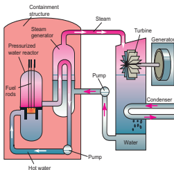
FIGURE 19.24 Pressurized water nuclear reactor. Water is superheated and pressurized as it flows through the reactor core. Heat is transferred to nonpressurized water in the steam generator. The steam drives the turbogenerator to produce electricity.
