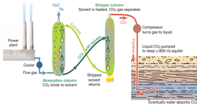
FIGURE 15.27 One method of carbon capture and storage uses a liquid solvent, such as ammonia, to capture CO 2 . Steam and nitrogen are released, and the CO 2 is compressed and pumped to deep aquifers for permanent storage.
