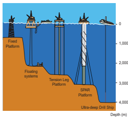
Types of drilling rigs. Note that the rigs aren't drawn to scale. The cylindrical spar, for example is about 200 m tall, while the drill rig below it reaches down as much as 10,000 m.
