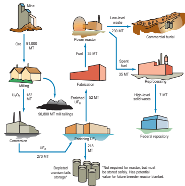
FIGURE 19.22 The nuclear fuel cycle. Quantities represent the average annual fuel requirements for a typical 1,000 MW light water reactor (MT = metric tons). About 35 MT, or one-third of the reactor fuel, is replaced every year. Reprocessing is not currently done in the United States.
