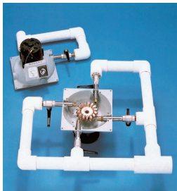
FIGURE 20.27 Solar collectors capture power only when the sun shines, but hydropower is available 24 hours a day. Small turbines such as this one can generate enough power for a single-family house with only 15 m (50 ft) of head and 200 l (50 g) per minute flow. The turbine can have up to four nozzles to handle greater water flow and generate more power.
