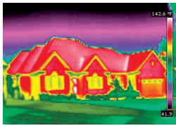
FIGURE 20.5 Infrared photography shows heat loss in a building.
