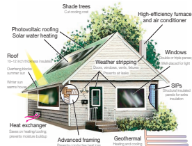
FIGURE 20.6 Energy-efficient buildings can lower energy costs dramatically. Many features can be added to older structures. New buildings that start with energy-saving features (such as SIPs or advanced framing) can save even more money.
