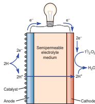
FIGURE 20.16 Fuel cell operation. Electrons are removed from hydrogen atoms at the anode to produce hydrogen ions (protons) that migrate through a semipermeable electrolyte medium to the cathode, where they reunite with electrons from an external circuit and oxygen atoms to make water. Electrons flowing through the circuit connecting the electrodes create useful electrical current.
