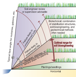
FIGURE 13.32 Steep streambanks need to be reinforced or recontoured to avoid erosion. Shallow slopes can be stabilized with vegetation or mulch. Steeper slopes need stabilization structures or reinforcement to hold the soil.
