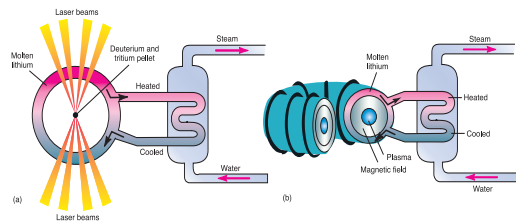
FIGURE 19.28 Nuclear fusion devices. (a) Inertial confinement is created by laser beams that bombard and ignite fuel pellets. Molten lithium transfers heat to a steam generator. (b) In the tokamak design, a powerful magnetic field confines the plasma and compresses it so that critical temperatures and pressures are reached.
