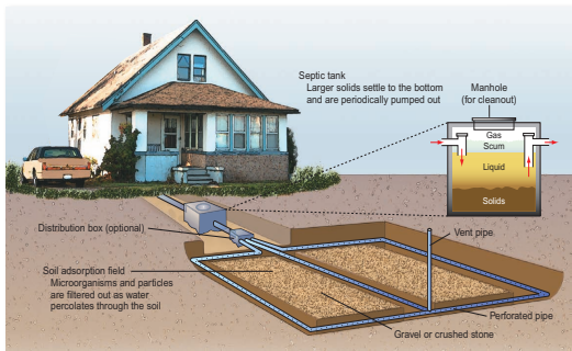
FIGURE 18.22 A domestic septic tank and drain field system for sewage and wastewater disposal. To work properly, a septic tank must have healthy microorganisms, which digest toilet paper and feces. For this reason, antimicrobial cleaners and chlorine bleach should never be allowed down the drain.
