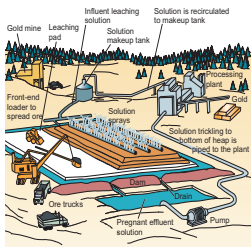
FIGURE 14.14 In a heap-leach operation, huge piles of low-grade ore are heaped on an impervious pad and sprayed with a cyanide solution. As the leaching solution trickles through the crushed ore, it extracts gold and other precious metals. This technique is highly profitable but carries large environmental risks.
