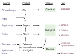
FIGURE 20.21 Methods for turning biomass into fuel.
