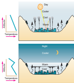
FIGURE 16.12 Atmospheric temperature inversions occur where ground-level air cools more quickly than upper levels. This temperature differential prevents mixing and traps pollutants close to the ground.
