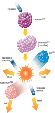
FIGURE 19.23 The process of nuclear fission is carried out in the core of a nuclear reactor. In the sequence shown here, the unstable isotope, uranium-235, absorbs a neutron and splits to form tin-131 and molybdenum-103. Two or three neutrons are released per fission event and continue the chain reaction. The total mass of the reaction product is slightly less than the starting material. The residual mass is converted to energy (mostly heat).
