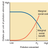
FIGURE 23.20 To achieve maximum economic efficiency, regulations should require pollution prevention up to the optimum point ( P_0 ) at which the costs of eliminating pollution just equal the social benefits of doing so.
