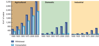
FIGURE 17.12 Growth of water withdrawal and consumption, by sector, with projected levels to 2025. Source: UNEP, 2002.
