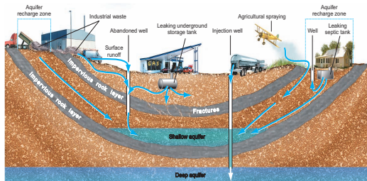
FIGURE 18.18 Sources of groundwater pollution. Septic systems, landfills, and industrial activities on aquifer recharge zones leach contaminants into aquifers. Wells provide a direct route for injection of pollutants into aquifers.
