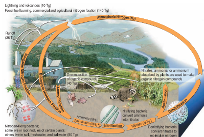
FIGURE 3.21 The nitrogen cycle. Human sources of nitrogen fixation (conversion of molecular nitrogen to ammonia or ammonium) are now about 50 percent greater than natural sources. Bacteria convert ammonia to nitrates, which plants use to create organic nitrogen. Eventually, nitrogen is stored in sediments or converted back to molecular nitrogen ( 1 \text{ Tg} = 10^{12} \text{ g} ).
