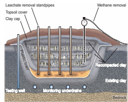
FIGURE 21.23 A secure landfill for toxic waste. A thick plastic liner and two or more layers of impervious compacted clay enclose the landfill. A gravel bed between the clay layers collects any leachate, which can then be pumped out and treated. Well samples are tested for escaping contaminants and methane is collected for combustion.
