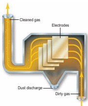
FIGURE 16.24 An electrostatic precipitator traps particulate matter on electrically charged plates as effluent makes its way to the smokestack.
