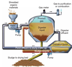
FIGURE 20.19 Continuous unit for converting organic material to methane by anaerobic fermentation. One kilogram of dry organic matter will produce 1–1.5 m 3 of methane, or 2,500–3,600 million calories per metric ton.
